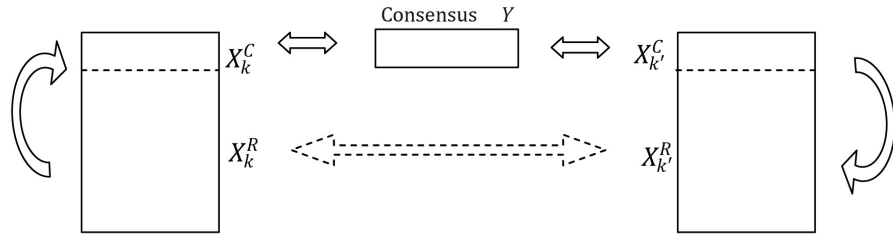
Figure 2: Flow scheme for comparing individuals in each condition through the consensus of individuals in common.
