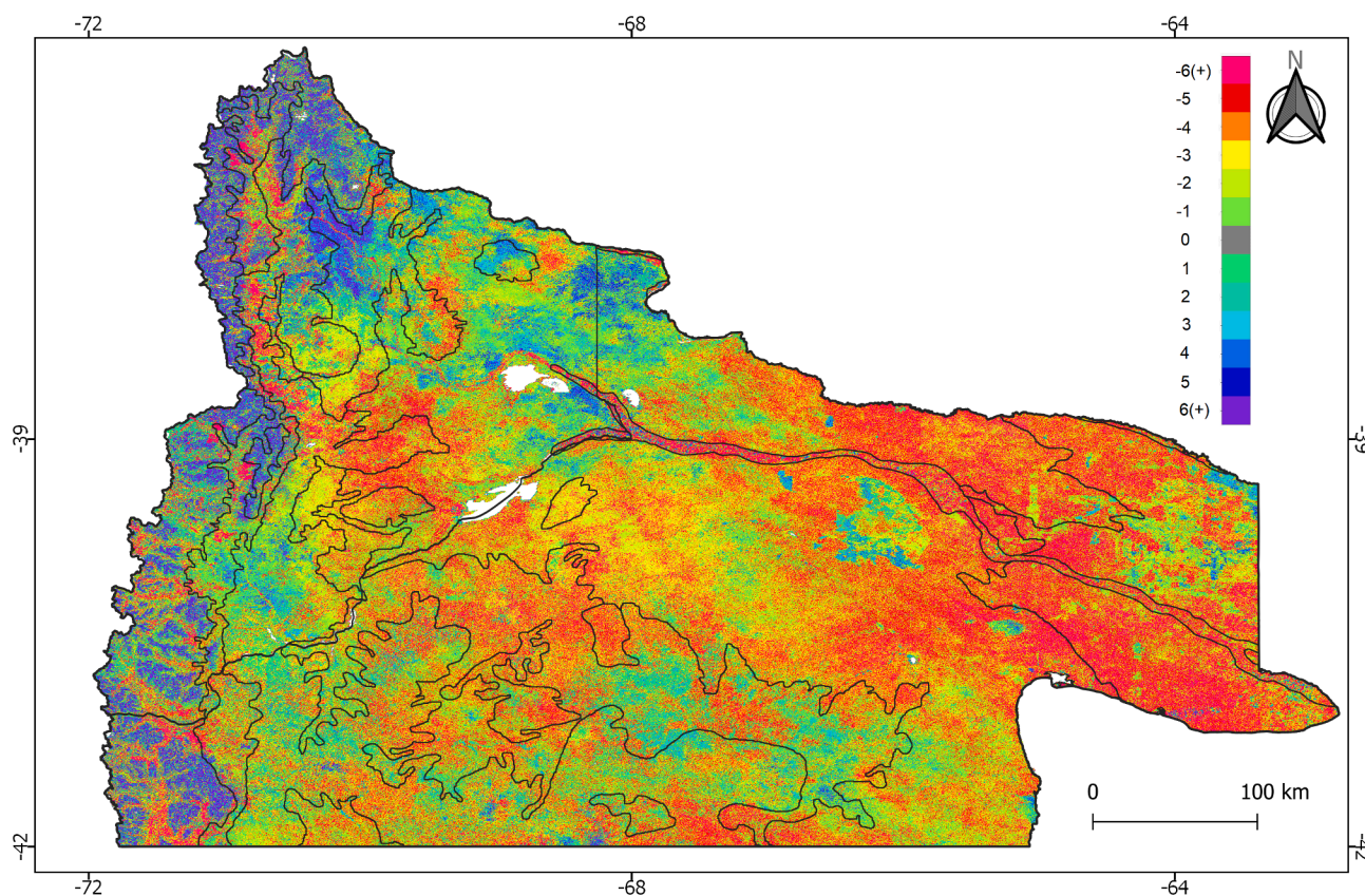
Fig. 7. Expected time (years) for the NDVI trend-cycle to reach the next minimum or maximum values, depending on the kind of movement: downward (negative values) or upward (positive values). Data source: MODIS images for the time series between 2000-mid-2020.
