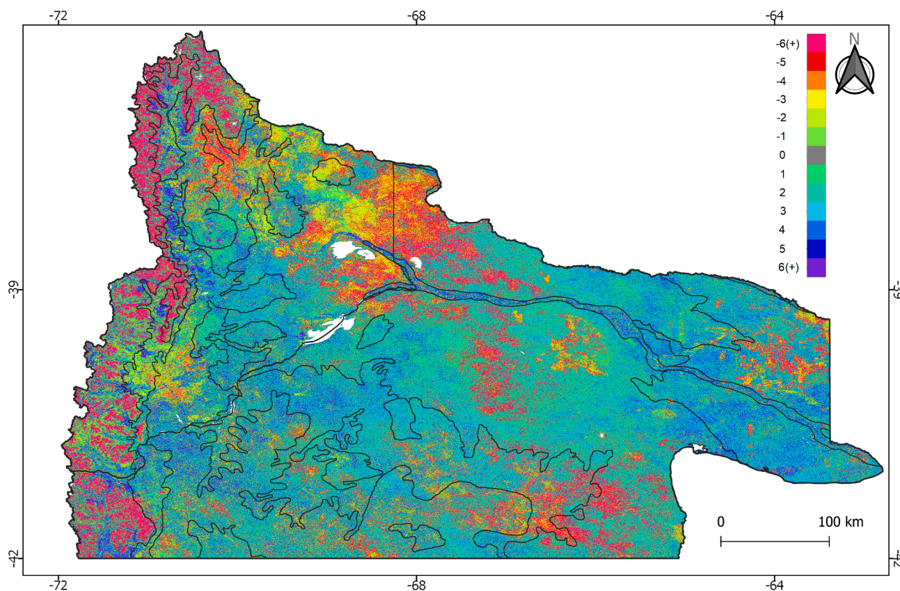
Fig. 6. Expected time (years) for the NDVI trend-cycle to reach the average of the time series (see Fig. 3). References: Current values below the average, but with an upward movement (negative values, color gradient green-yellow–red), and current values above the average, but with a downward movement (positive values, color gradient turquoise-blue-violet). Data source: MODIS images for the time series between 2000–mid-2020. (For interpretation of the references to color in this figure legend, the reader is referred to the web version of this article.)
