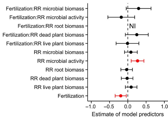
FIGURE 4 Plots showing the parameter estimates of the potential local controls explaining the response ratios (RR) of soil C (a, c) and N pools (b, d) to herbivore exclusion. The parameters are response ratios of plant biomass (live, dead and root) and microbial properties (biomass, activity) to herbivore exclusion. Parameter estimates were generated by multi-model inference, which uses model averaging to arrive at consistent parameter estimates of the most important explanatory variables. Models included fertilization as a fixed factor (under fertilization the effect of herbivore exclusion is negative; also see Figure 3) and interactions are presented as 'Fertilization:other parameter'. Models were run without (22 sites, n = 126 ; a, b) and with (12 sites, n = 67 ; c, d) microbial data. Points represent the mean value of the model predictor while error bars represent the range of 95% confidence intervals. Predictors are considered significant if error bars do not overlap with zero and are coloured red. NI indicates the variable was not included in the set of top models
