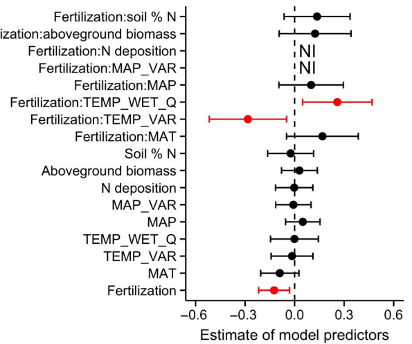
FIGURE 5 Plots showing the parameter estimates of the potential environmental drivers explaining the response ratios (RR) of soil C (a) and N pools (b) to herbivore exclusion. Parameter codes are: MAT, mean annual temperature; TEMP_VAR, temperature seasonality; TEMP_WET_Q, mean temperature of wettest quarter; MAP, mean annual precipitation; MAP_VAR, precipitation seasonality; aboveground biomass and soil % N are measures of in situ productivity and soil fertility. See Section 2 for more details. Parameter estimates were generated by multi-model inference, which uses model averaging to arrive at consistent parameter estimates of the most important explanatory variables. Models included fertilization as a fixed factor and interactions are presented as 'Fertilization:other parameter'. Points represent the mean value of the model predictor while error bars represent the range of 95% confidence intervals. Predictors are considered significant if error bars do not overlap with zero and are coloured red. NI indicates the variable was not included in the set of top models
