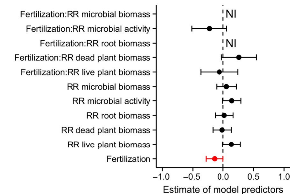
FIGURE 4 Plots showing the parameter estimates of the potential local controls explaining the response ratios (RR) of soil C (a, c) and N pools (b, d) to herbivore exclusion. The parameters are response ratios of plant biomass (live, dead and root) and microbial properties (biomass, activity) to herbivore exclusion. Parameter estimates were generated by multi-model inference, which uses model averaging to arrive at consistent parameter estimates of the most important explanatory variables. Models included fertilization as a fixed factor (under fertilization the effect of herbivore exclusion is negative; also see Figure 3) and interactions are presented as 'Fertilization:other parameter'. Models were run without (22 sites, n = 126 ; a, b) and with (12 sites, n = 67 ; c, d) microbial data. Points represent the mean value of the model predictor while error bars represent the range of 95% confidence intervals. Predictors are considered significant if error bars do not overlap with zero and are coloured red. NI indicates the variable was not included in the set of top models
