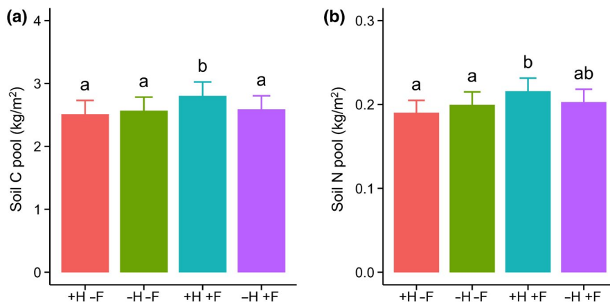
FIGURE 2 Effect of herbivore exclusion (+H: herbivores present; -H: herbivores excluded) and fertilization (+F: fertilized with NPK \mu ; -F: unfertilized) on soil C (a) and N pools (b). Shown are sample means \pm SE. Different letters indicate significant differences among the treatment means
