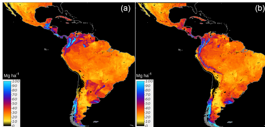
Figure 5. Country-specific (a) and regional (Latin America) (b) predictions of SOC based on a linear ensemble of methods. We present the units as Mg ha for visualization purposes. These units were used to reduce the digits of the value range and highlight larger differences between SOC maps.
