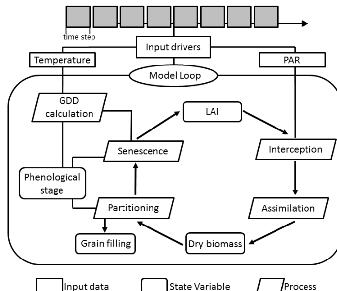
Figure 17. GRAMI model flowchart (adapted from Delécolle, 1992 and Ko et al, 2005).
