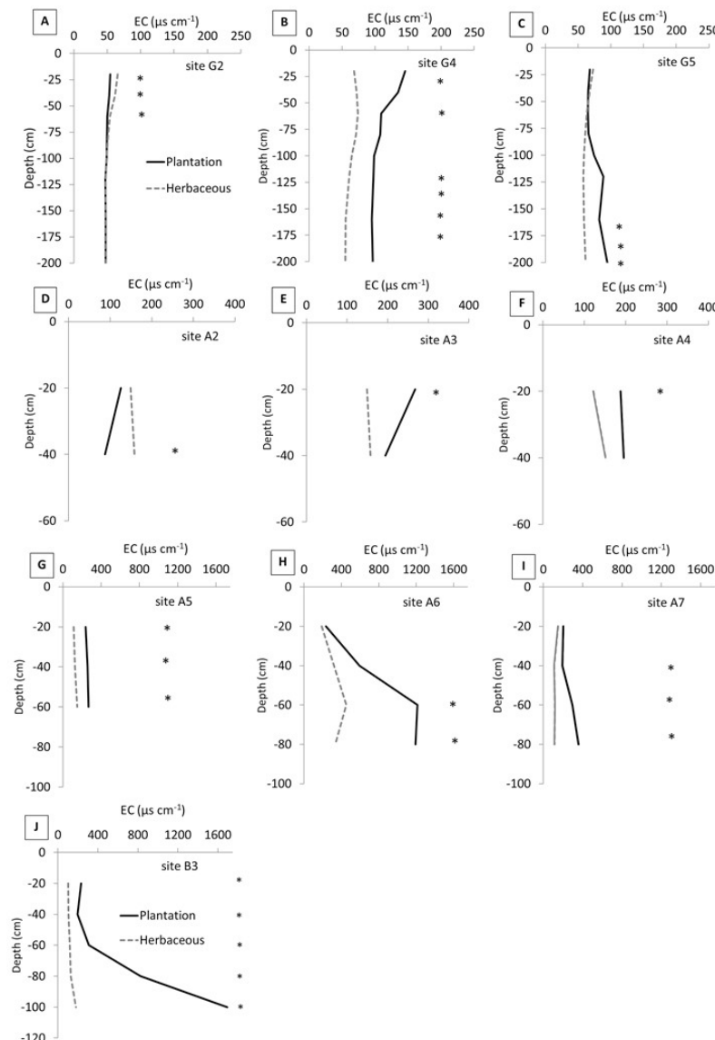
FIGURE 1 Soil electrical conductivity (EC, \mu\text{S cm}^{-1} ) at different sampling depths in plots covered by herbaceous vegetation (crops and grasslands) and Eucalyptus spp. in districts: Guaminí (panels A to C), Azul (panels D to I) and Balcarce-Lobería (panel J). Only the 10 plots in which statistical differences in at least one soil layer are depicted. Asterisks denote significant differences between soils layers between the two vegetation types in each site ( P < 0.05 ).
