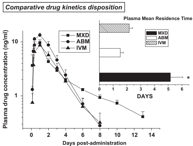
Fig. 1. Mean ( \pm SD) ( n = 6 ) moxidectin, (MXD), abamectin (ABM) and ivermectin (IVM) plasma concentrations obtained after their intraruminal (IR) administration (0.2 mg/kg) to nematode infected lambs. The insert shows the comparative plasma mean residence time obtained for the three compounds under study. (*) Values for MXD are statistically different from those obtained after the administration of ABM and IVM at P < 0.05 .
