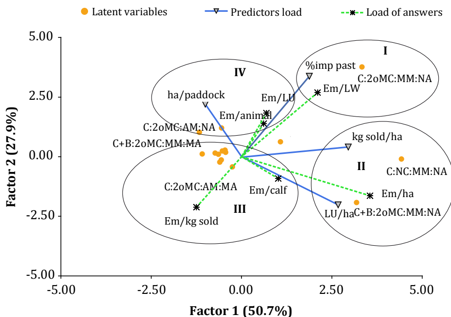
Figure 1. Triplot of the correlation between the interaction matrix of dependent variables (emissions), latent variables (system factors) and predictors (system characteristics). Load of answers: Em/animal: animal emissions. Em/calf: calf emissions. Em/kg sold: kg sold emissions. Em/LU: livestock unit emissions. Em/LW: animal live weight emissions. Em/ha: hectare emissions. Latent variables: C: cow-calf. B: backgrounding. C+B: cow-calf + backgrounding. NM: None management. MM: moderate management. AM: Appropriate management. NA: No technical advice. MA: Moderate technical advice. GA: good technical advice. NC: no control. 1C: 1 control. 2 o MC: 2 or more controls. Predictors load: % impl past; ha/paddock; LU/ha; kg sold/ha.
