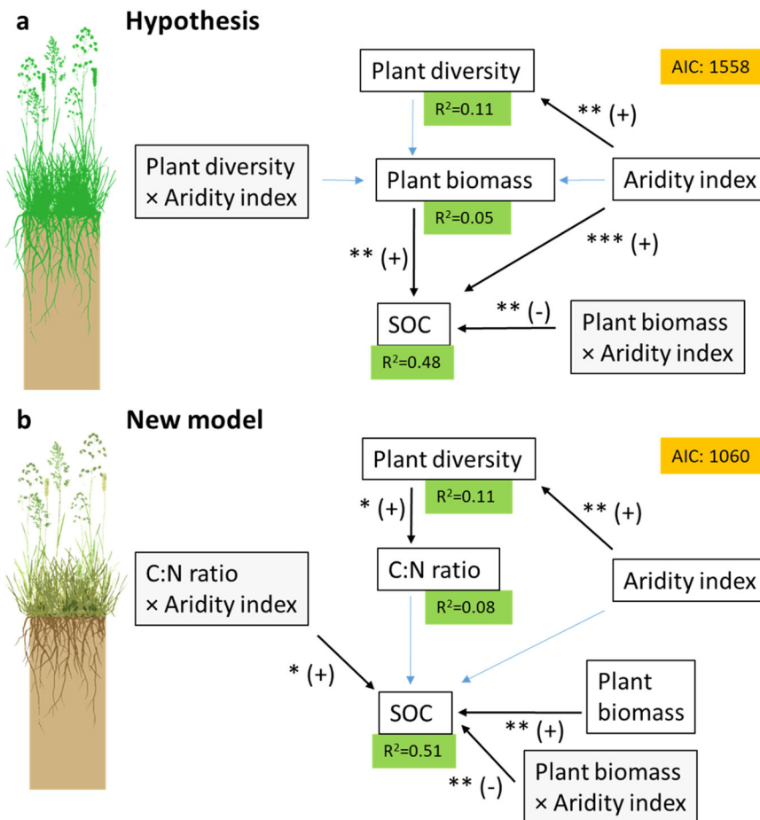
Fig. 1 | Two structural equation models depicting the original hypothesis and the new, optimized model. The initial hypothesis (a) states that plant diversity affects SOC through the quantity of organic matter (plant biomass) inputs to soil, whereas the new model (b) states that plant diversity affects SOC through the quality of organic matter (C:N ratio). Quality of plant organic matter is depicted in the drawing of the grassland in panel b by different colors. Gray boxes show interactions. Black arrows indicate significant regressions. Asterisks indicate the level of significance of the regressions ( P < 0.05 , ^*P < 0.01 , ^{***}P < 0.001 ), and (+) and (-) indicate whether the slope of the linear regression model is positive or negative.
