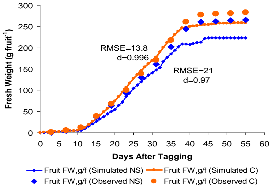
Figure 7- 25. CROPGRO simulated (line) vs. observed (points) fresh weight of individual fruits of cohort # 1 in Gainesville Fl, during spring 2007 comparing well fertilized with N stressed tomato plants.
