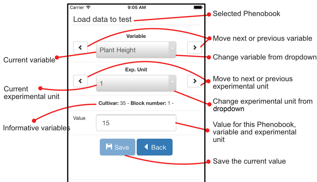
Figure 2: A screenshot of Phenobook mobile.
