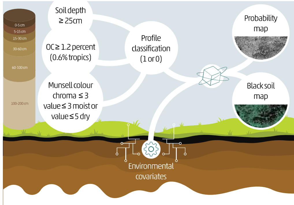
Figure 2.2 Workflow for mapping black soils
