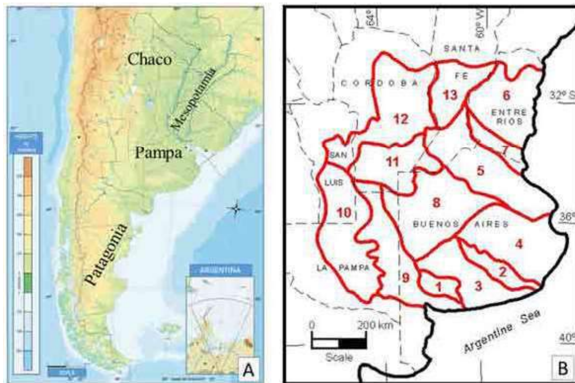
Figure 2.5 Distribution of main ecological regions in Argentina
