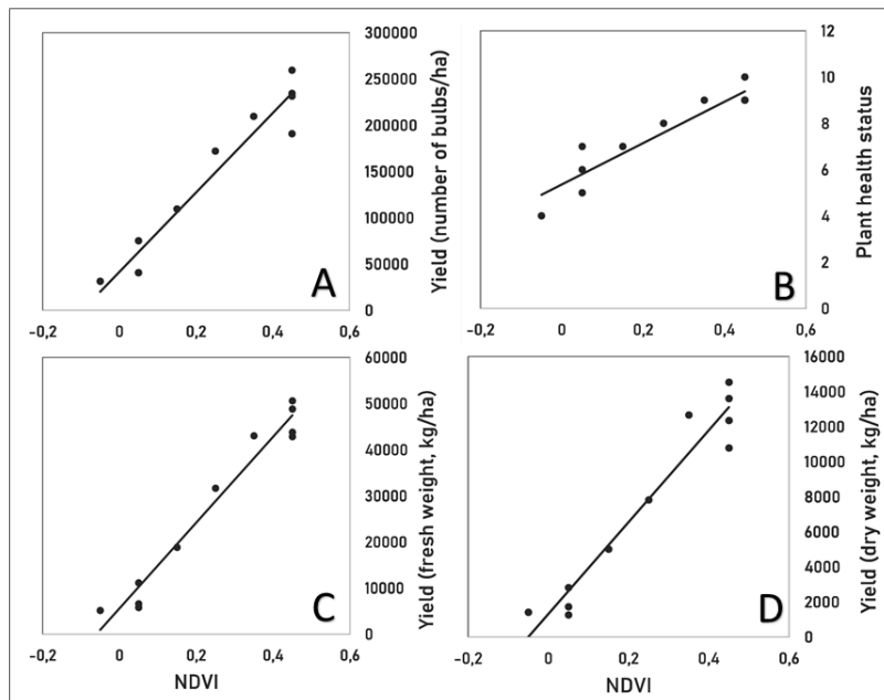
Fig. 1. NDVI as predictor of different yield and health aspects in a garlic crop. Fig. A: number of harvested bulbs; Fig. B: health status of the plot; Fig. C: fresh weight at harvest; Fig. D: dry yield. Date of data acquisition: 8 October 2020.
